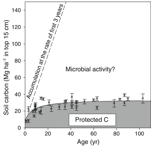
Fig. 11.2 Comparison of the actual pattern of soil carbon accumulation with that extrapolated from the initial rate of accumulation (3 years) for bermudagrass turf in North Carolina, USA
